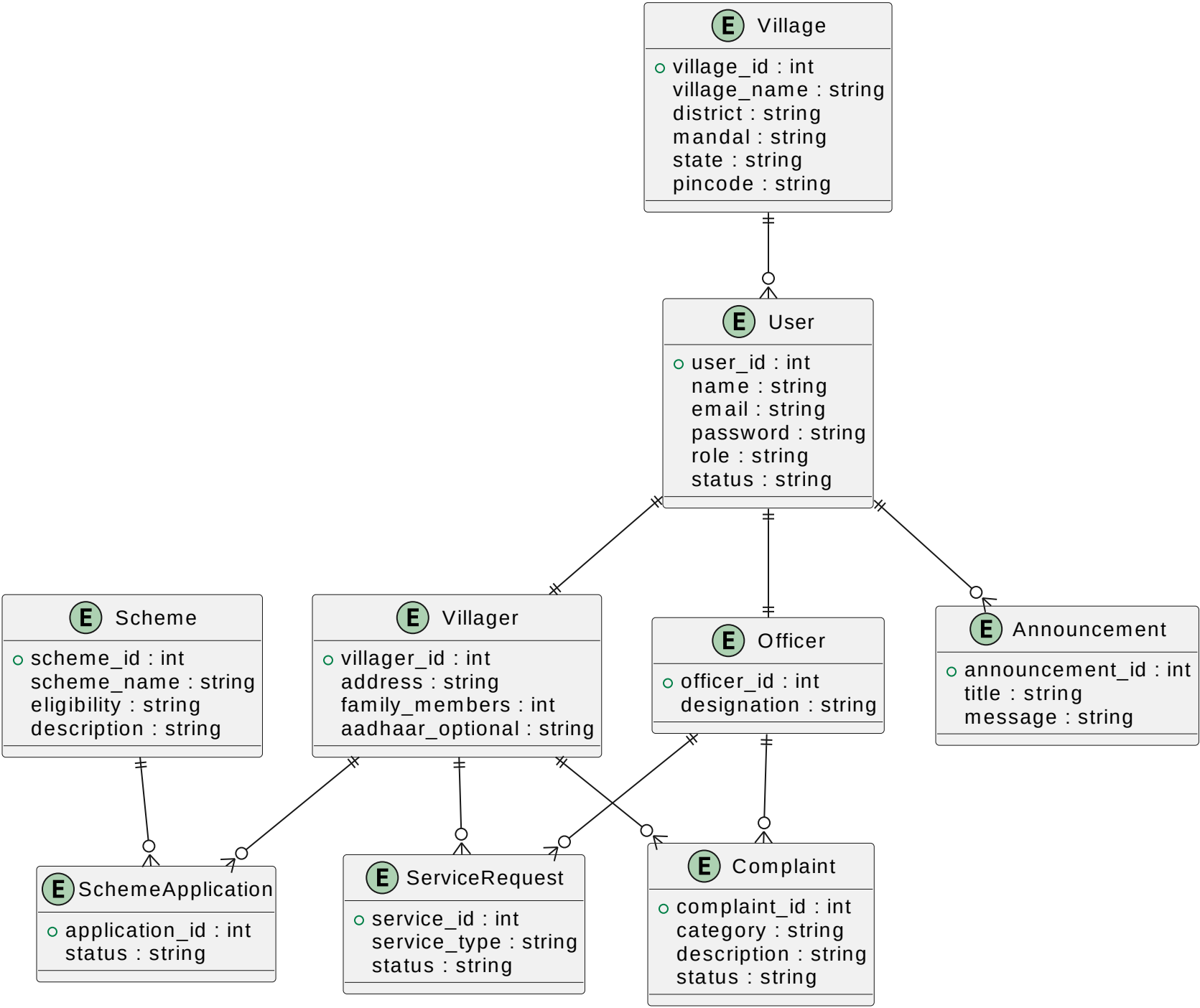
ER Diagram - Digital Village Management System (DVMS)
